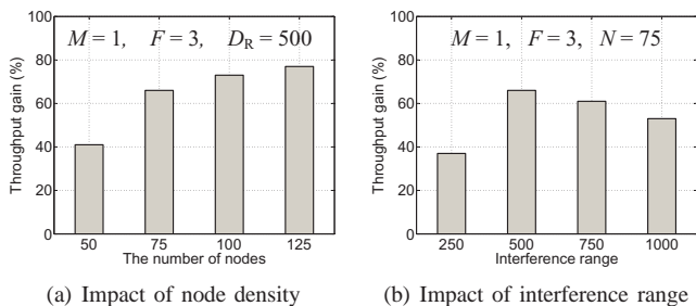
Fig. 10. The average throughput gain of IN versus node density and interference range, where M is the number of antenna, N is the total number of nodes, F is the number of sessions, and D_R is the interference range.
