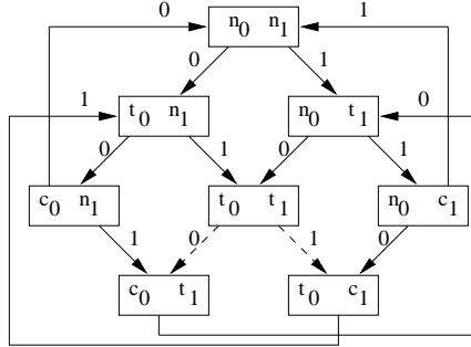
Fig. 4. The reachability graph of program ME .
