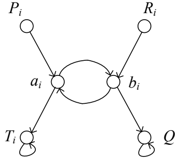
Fig. 2. Mapping of variables in the 3-SAT problem.
