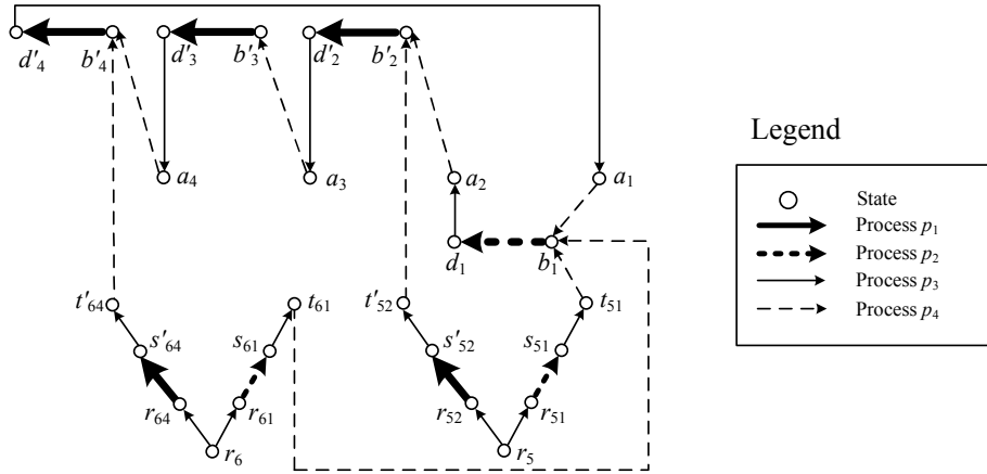
Fig. 2. The structure of the revised program for Boolean formula (x_1 \vee \neg x_2 \vee x_3) \wedge (x_1 \vee x_2 \vee \neg x_4) , where x_1 = \text{true} , x_2 = \text{false} , x_3 = \text{false} , and x_4 = \text{false} .
