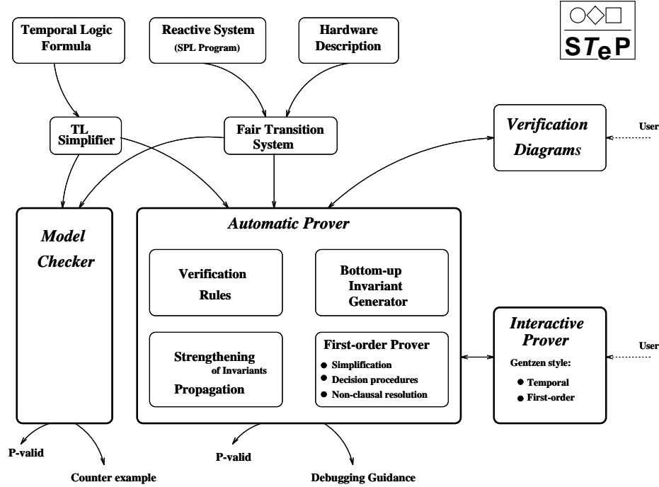
Fig. 1. An overview of the STeP system
