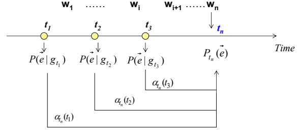
Figure 3: Saliency modeling: the saliency distribution at time t_n is calculated by a joint effect of gestures that happen before t_n .
