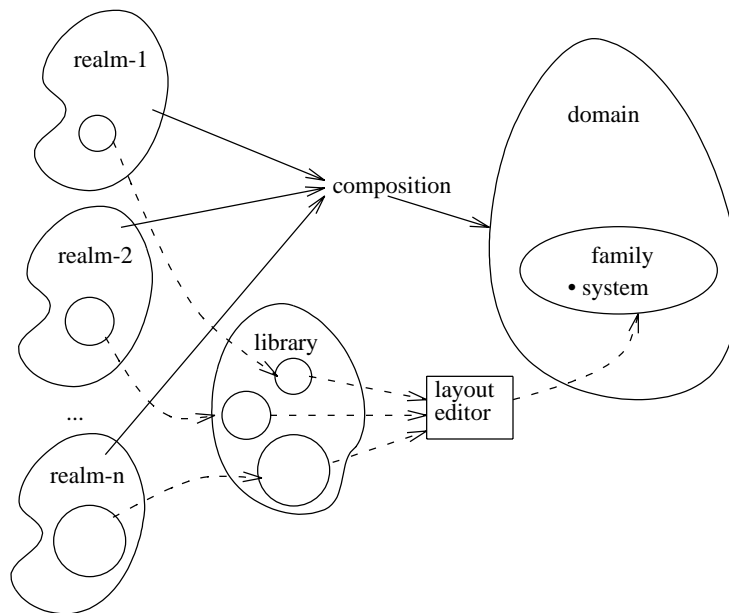
Figure 2.2 Realms, Libraries, Composition, Layout Editor, Family of Systems, and Domain
