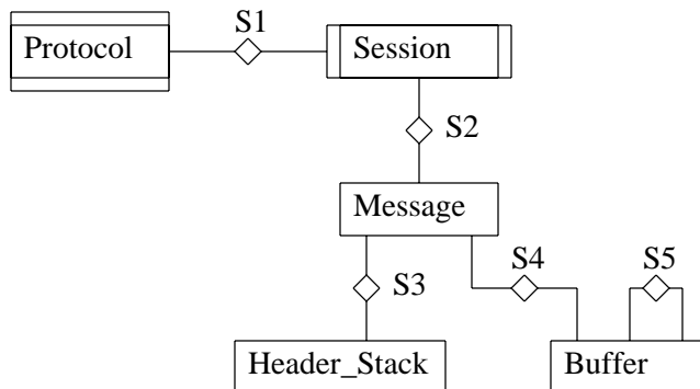
Figure 4.5 The ASYNC Object Model Interface
