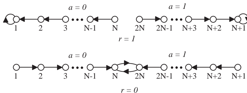
Figure 3: A Tsetlin automaton with 2N states. The top row shows the state transitions that are made when the previous action resulted in a reward of 1; the bottom row shows transitions after a reward of 0. In states in the left half of the figure, action 0 is taken; in those on the right, action 1 is taken.
