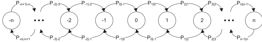
Fig. 3. \mathcal{RW} -1: One-dimensional random walk
